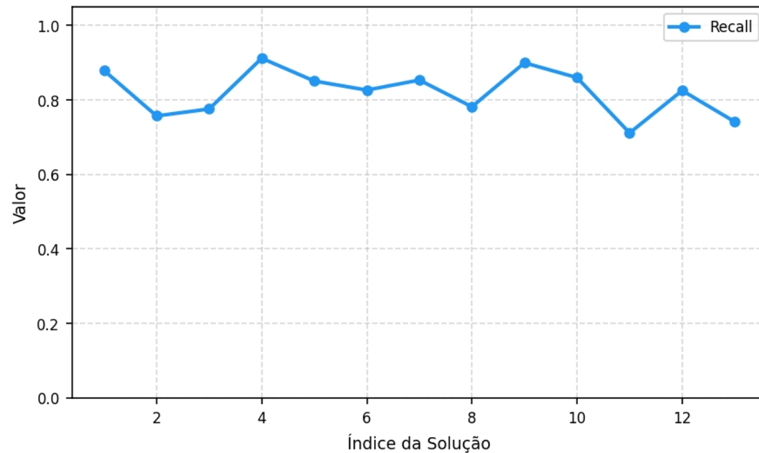
Generalization
