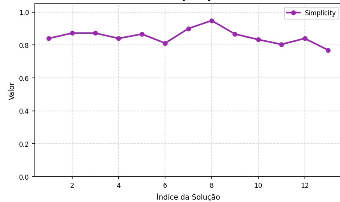
Simplicity
