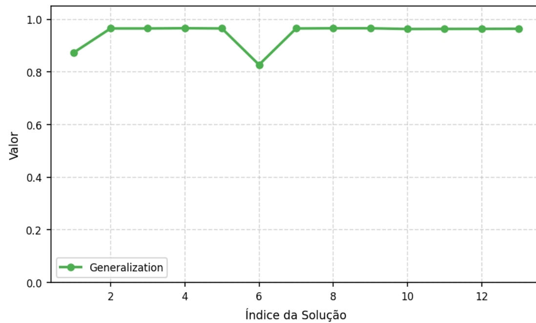
Generalization
